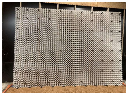
4-point support configurator Backside of the full CircoFloor structure (12m²) with 98 supports
